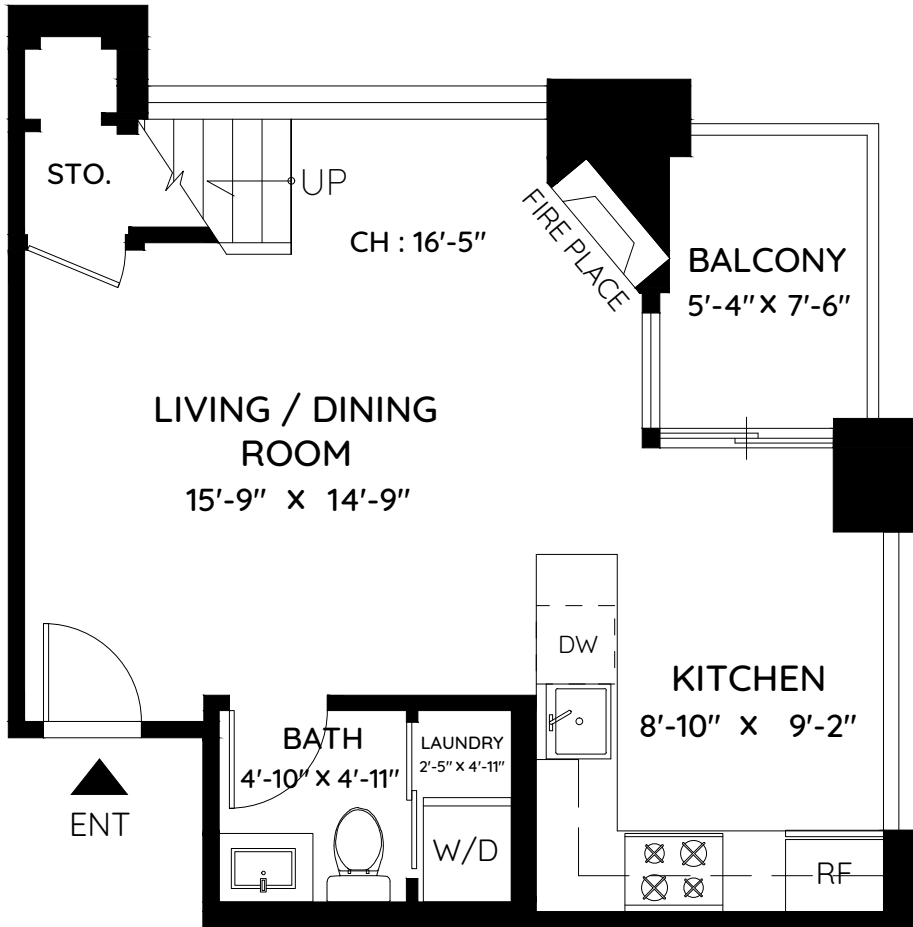
MAIN FLOOR 423 SQ.FT. CH: 8'-0"
