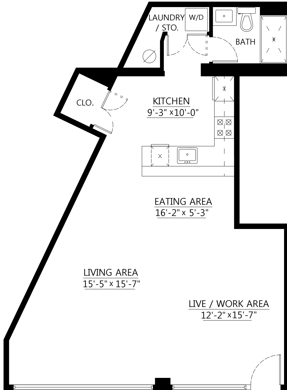
Main Floor Plan Floor Area: 809 sq.ft.
