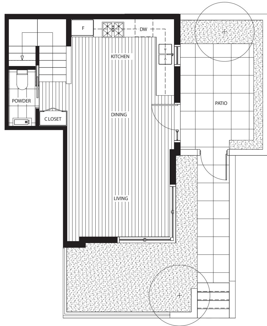
MAIN FLOOR
